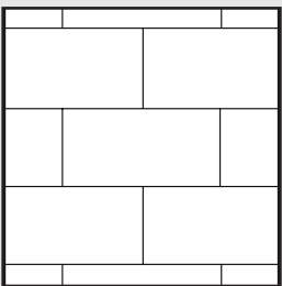
Fig. 3b Stone effect: Tiles should be fitted in a 'brick' pattern (off-set).
